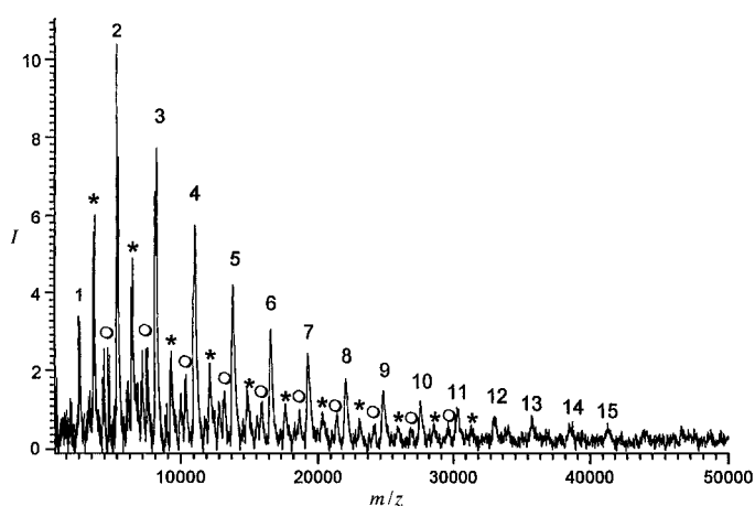
Figure 3. MALDI-TOF mass spectrum of poly[2]catenand 12b ( n refers to =(\text{spacer-catenand})_n with n=1,2,3 to 15; * refers to (\text{spacer-catenand})_n - \text{spacer} ; o refers to \text{catenand} - (\text{spacer-catenand})_n ).
