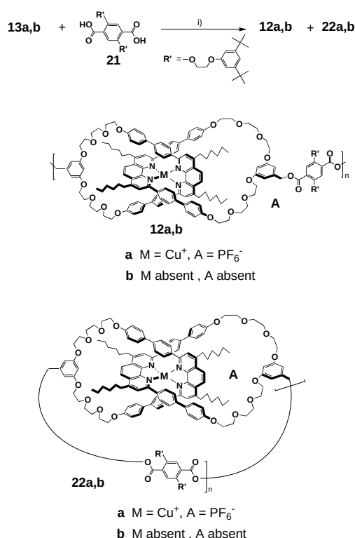
Scheme 8. Synthesis of oligo- and poly[2]catenates ( 12a , 22a ) and oligo- and poly[2]catenands ( 12b , 22b ). i) 4-( N,N' -dimethylamino)pyridine/ p -toluenesulfonic acid 1:1 complex, N,N' -diisopropylcarbodiimide.
