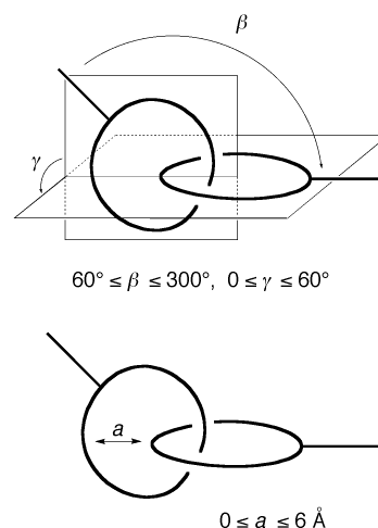
Figure 4. The mobility elements contained in catenane monomer units of 12b and 22b : rotational motions \beta and \gamma , and elongational motion a .
