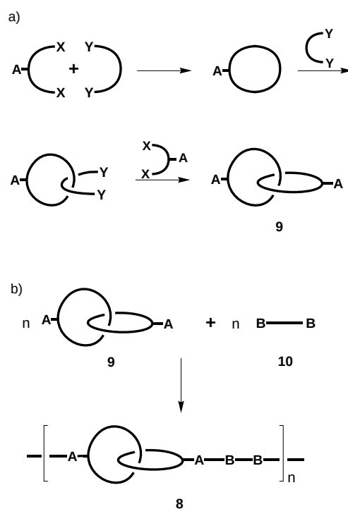
Scheme 2. Synthetic strategy leading to poly[2]catenane 8 .
