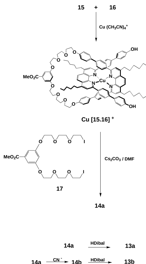
Scheme 5. Synthesis of catenate monomer 13a and catenand monomer 13b .
