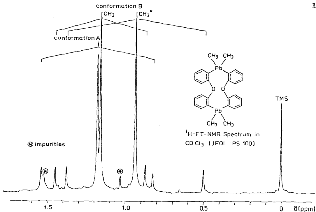
Fig. 3. 1 H NMR spectrum of compound III.
