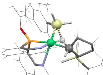
Fig 4 Transition state TS2 for reaction of \text{PhSiH}_3 with [(\text{NPN})\text{Ni}(\text{C}_5\text{H}_9)\text{SiH}_2\text{Ph}]^+ . The atoms involved in the reaction (Si, H, Ni and C) are represented by sphere (green for Ni, yellow for Si, white for H and black for C). Other atoms are represented by stick and wire.
