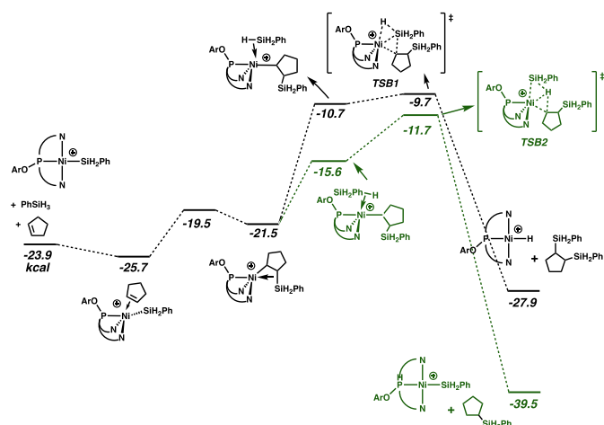
Fig. 3 Gibbs energy profile for cycle B of the hydrosilation catalyzed by [(NPN)NiSiH 2 Ph] + .
