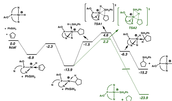
Fig 2 Gibbs energy profile (kcal mol ^{-1} ) for cycle A of the hydrosilylation catalyzed by [(NPN)NiH] ^+ .
