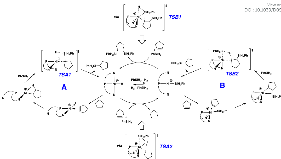
Scheme 3 Proposed Mechanisms for Nickel-Catalyzed Hydrosilylation of Alkenes.
