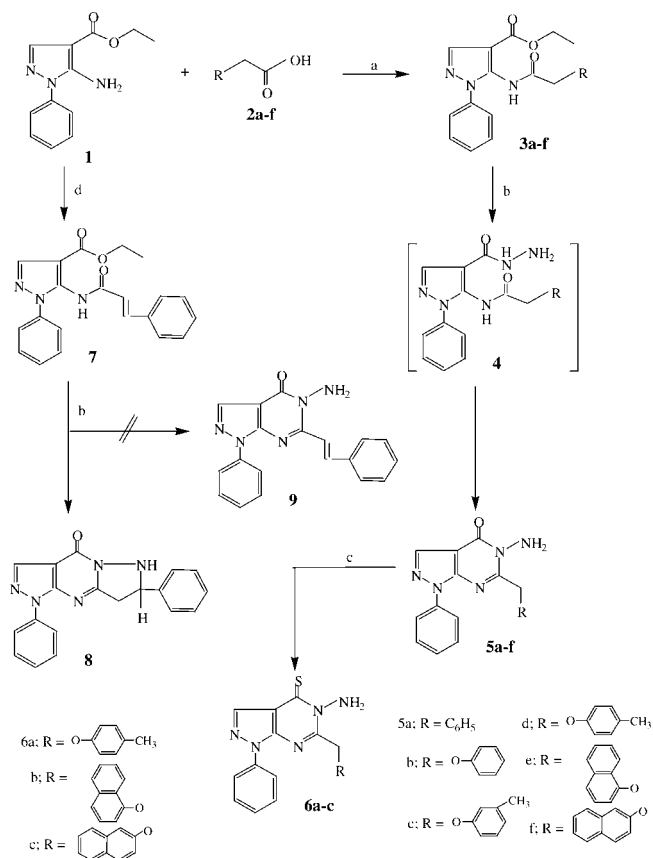
SCHEME 1 Synthesis of pyrazolopyrimidine derivatives ( 5a-f , 6a-c , and 8 ). a: PCl 3 /xylene, reflux, 5 h; b: N 2 N 4 ·H 2 O, n -BuOH, reflux 6 h; c: P 2 S 5 /pyridine, reflux 16 h; d: cinnamic acid/PCl 3 /xylene, reflux, 5 h.
