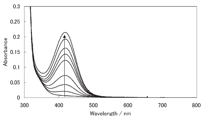
Figure 3. Change in absorption spectrum of 8R in toluene at 26 °C ( 1.00 \times 10^{-4} mol dm ^{-3} ). Irradiation time/s; 0, 20, 60, 120, 240, 300, 420, 600, 960. Light intensity; 0.68 mW cm ^{-2} (313 nm). Cell length; 1 cm
