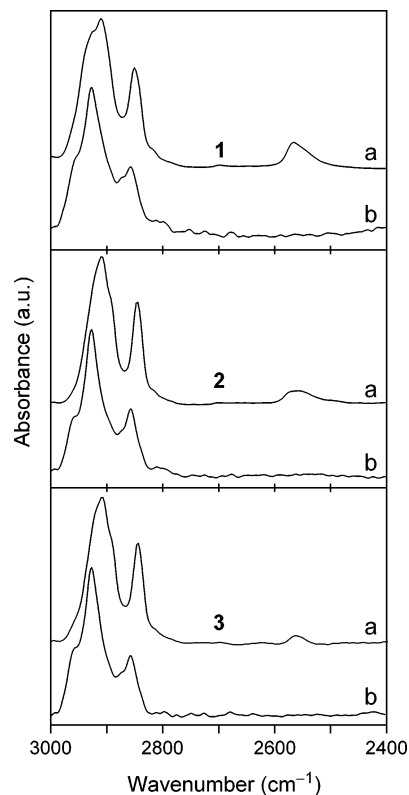
FIGURE 2. Infrared absorption spectra of trithiols 1–3 . (a) Transmission spectra of neat samples on a KBr plate. The sample was prepared by dropping a 5 mM solution of the compound in ethyl ether on a plate and slowly evaporating the solvent. The dropping and evaporation were repeated five times. (b) PM-IRRAS spectra of the monolayers on Au(111).
