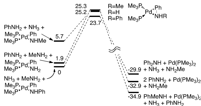
Figure 1. Relative ground state and transition state free energies in kcal/mol for \text{PMe}_3 -ligated phenylpalladium parent amido, arylamido, and methylamido complexes undergoing C–N reductive elimination.
