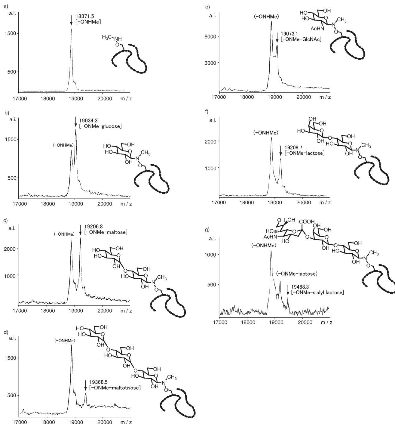
Figure 3. MALDI-TOF MS analysis of the molecular weight of mutant streptavidin and glycoprotein mimetics: a) mutant streptavidin having an unnatural amino acid 1 ; product obtained by glycoblotting of mutant streptavidin with b) glucose, c) maltose, d) maltotriose, e) N -acetylglucosamine, f) lactose; g) modification of the mutant streptavidin with glycosyltransferase.
