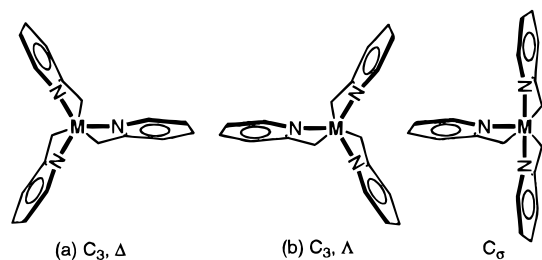
Figure 1. [M(TPA)]^{n+} C_3 and C_0 conformations. View is down the metal-tertiary amine axis.
