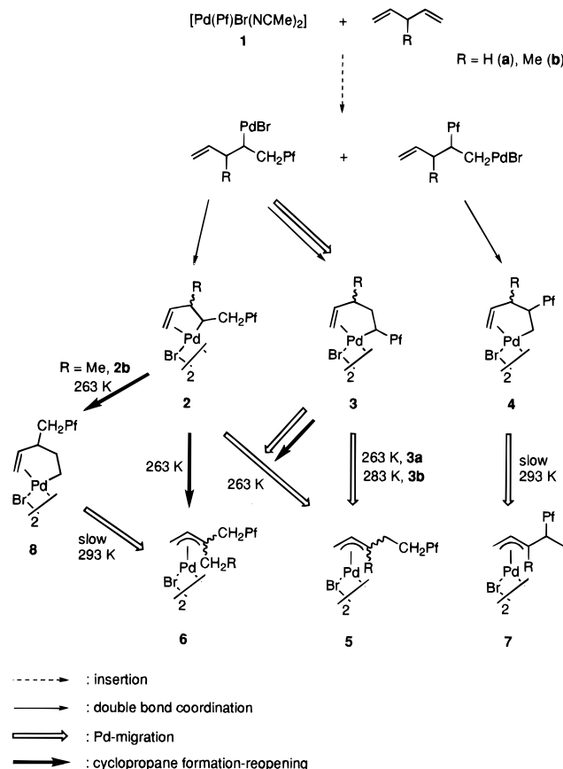
Scheme 3
