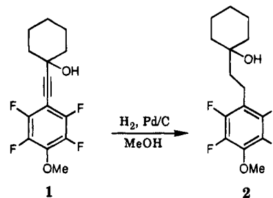
Figure 1. Phenylproparginol nucleus.
