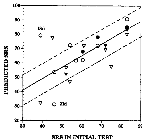
Figure 6. Predicted scaled rank sums (SRS) as a function of actual values in the initial test. Solid symbols (●, ▼) indicate predictions based on individual compounds included in both tests, whereas open symbols (○, ▽) indicate predictions based on regression models: (●, ○) \text{SRS}_{\text{BYGR}} ; (▼, ▽) \text{SRS}_{\text{DOBR}} . The solid line corresponds to eq 8; the dashed lines correspond to an error range of \pm 10 .
