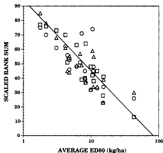
Figure 5. Scaled rank sums as a function of average weed ED 80 : (○) SRS BYGR ; (Δ) SRS DOBR ; (□) SRS YENS .
