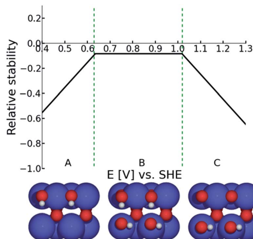
Fig. 9 Surface Pourbaix diagram for RuO 2 . Detailed description of the diagram construction is given in the ESI.†
