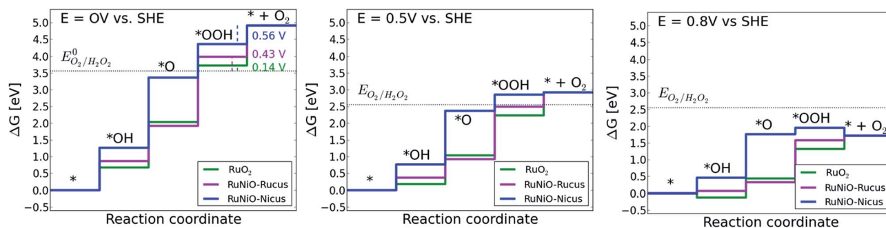
Fig. 11 Free energy diagrams for the reduction of O 2 on three catalytic active sites, the Ru cus site on conventional ruthenia (green), the cus Ru site on Ni doped RuO 2 (magenta) and the cus Ni site on Ni doped RuO 2 (blue). The dotted line represents the equilibrium potential of the reduction O 2 to H 2 O 2 . The key difference is the binding of O on the Ni cus site compared to the Ru cus sites.
