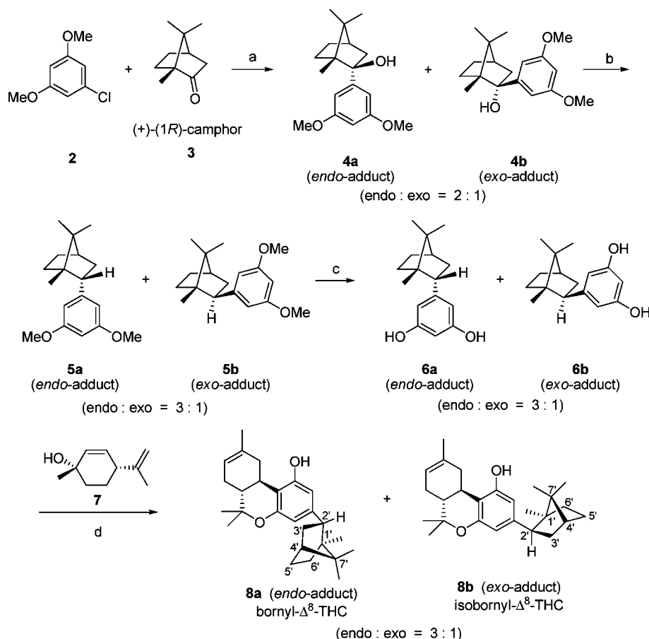
Scheme 1. Synthesis of Bornyl- and Isobornyl- \Delta^8 -THC ( 8a and 8b ) a
