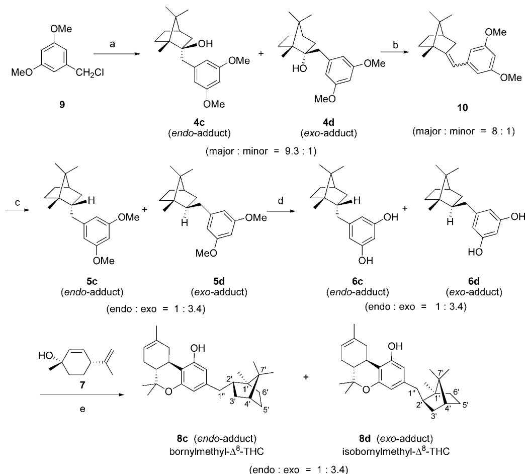
Scheme 2. Synthesis of Bornylmethyl- and Isobornylmethyl- \Delta^8 -THC ( 8c and 8d ) a
