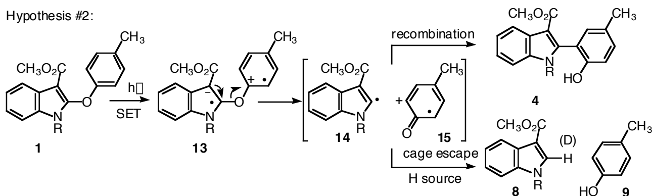
Scheme 4. Two mechanistic hypothesis for the rearrangement of 1 into 4 .
