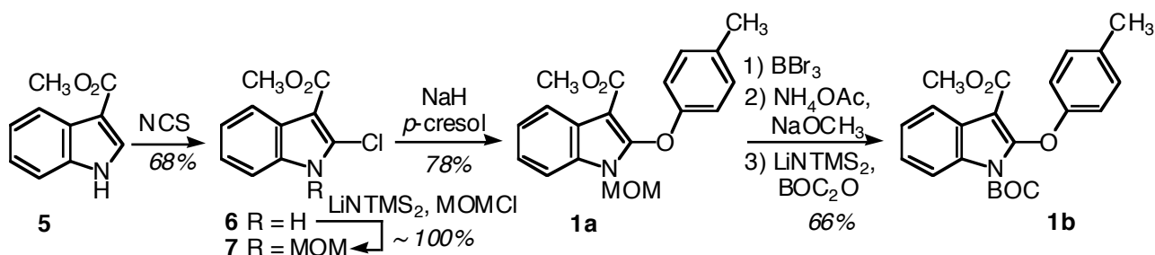
Scheme 2. Synthesis of substrates ( 1a ) and ( 1b ).
