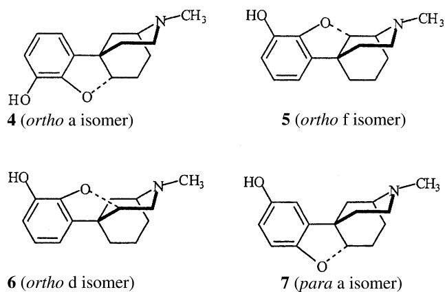
Fig. 2. Structures of previously synthesized epoxy-bridged isomers
