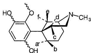
Fig. 1. Possible epoxy-bridged 5-phenylmorphans ( ortho or para (a–f) isomers)
