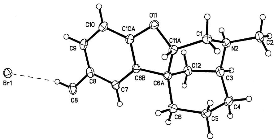
Fig. 3. X-Ray crystal structure of rac-(3R,6aS,11aR)-1,3,4,5,6,11a-hexahydro-2-methyl-2H-3,6a-methanobenzo furo[2,3-c]azocin-8-ol ( 3 ) (drawn from the experimentally determined coordinates with displacement ellipsoids at the 20% probability level)
