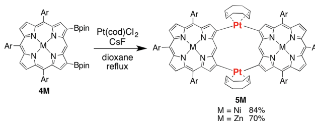
Scheme 2 Synthesis of doubly platinum-bridged porphyrin dimer 5M .
