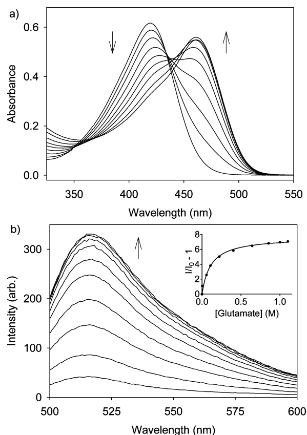
Figure 3. (a) Absorbance and (b) fluorescence titration of ES517 (20 \mu\text{M} ) in buffer (50 mM bis-tris propane, 50 mM \text{Na}_2\text{S}_2\text{O}_3 , 1% DMSO, pH 7.4) adding 20–800 \mu\text{L} aliquots of 1.5 M glutamate. \lambda_{\text{ex}} = 488 \text{ nm} . Inset is the fit to a binding isotherm.
