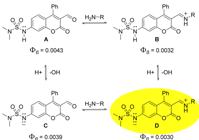
Scheme 1. Neurotransmitter Binding and Deprotonation of ES517 a
