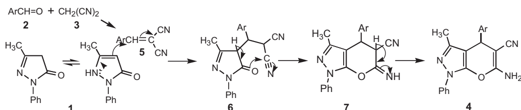
Scheme 2 Proposed mechanism for the formation of dihydro-pyranopyrazoles 4 .
