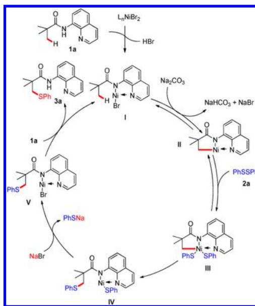
Scheme 5. Proposed Catalytic Mechanism
