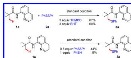
Scheme 4. Preliminary Mechanistic Study
