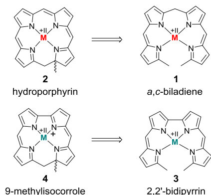
Figure 1 Strategies for hydroporphyrin and isocorrole syntheses.
