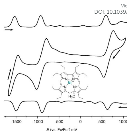
Figure 3 Cyclic voltammetry and square wave voltammetry results for nickel 9-methylisocorrole 7 (dichloromethane, 0.1 \text{ mol L}^{-1} n\text{Bu}_4\text{NPF}_6 ; scan rate 200 \text{ mV s}^{-1} ).
