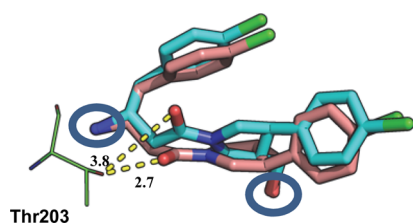
Figure 3. Overlay of 1b (cyan) and 2a (pink) bound in the peptide binding pocket of LmNMT obtained by alignment of the protein main chain atoms (distances in Å). PDB code for 2b : 4cyn.
