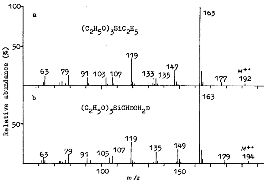
Fig. 4. Mass spectra of: (a) ethyl triethoxysilane; (b) 1,2-dideuteroethyltriethoxysilane.
