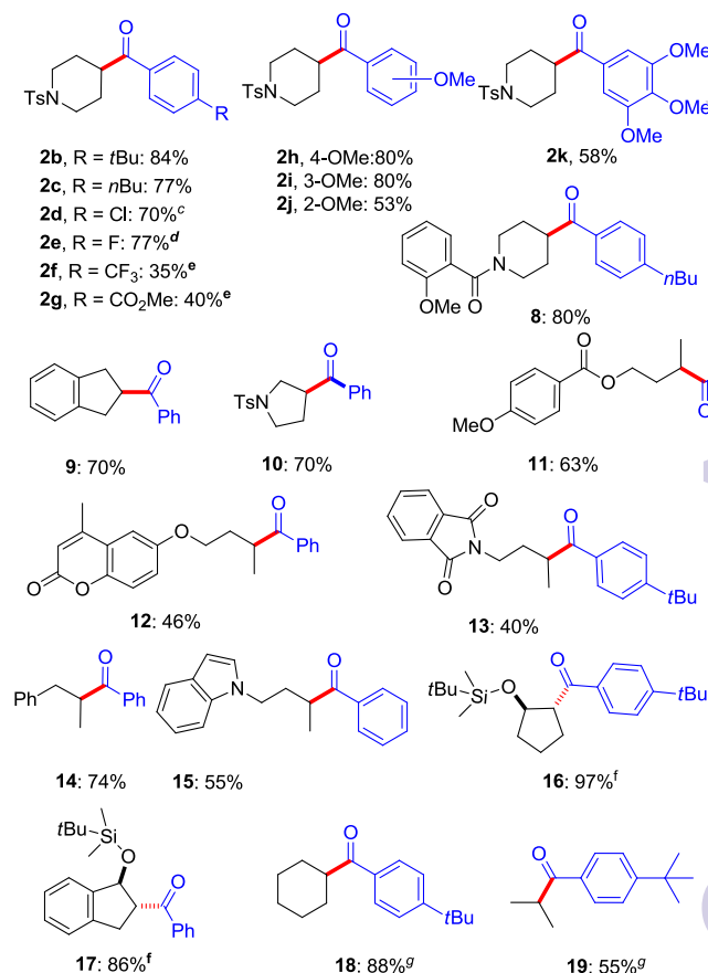
Figure 2. (a) Same as Table 1, entry 1. (b) Isolated yields. (c) DME/DMF = 1/9 (1 mL). (d) CN 3 CN/DMF (4/1, 0.5 mL). (e) 10% Ni(acac) 2 and 15% 4b were used. (f) dr > 20:1 (g) Alkyl iodide (0.3 mmol) was used under the reaction conditions in Table 2, entry 12 except CN 3 CN/DMF (4/1, 1 mL).
