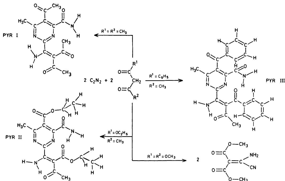
Scheme 1. The cyanation of \beta -dicarbonyl compounds catalysed by Ni(acac)_2 in C_2H_4Cl_2
