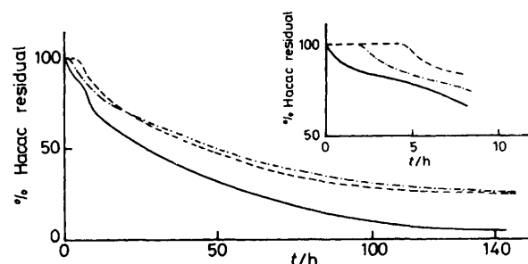
Figure 1. Plot of % residual Hacac versus time for different catalysts: [Hacac] 0.35M; [C_2N_2] 0.4M: — [Cu(acac)_2] 1.2 \times 10^{-3}M ; --- [Cu\beta_2] 1.2 \times 10^{-3}M ; - · - · - 1[Cu(acac)_2] + 1[Cu\beta_2] 1.2 \times 10^{-3}M
