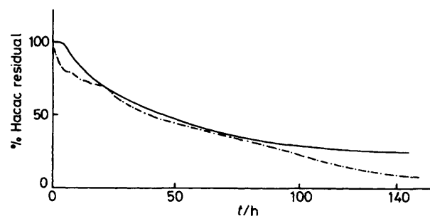
Figure 4. Effect of added H\alpha on the % residual Hacac versus time plot: [Cu\beta_2] 1.2 \times 10^{-3}M ; [Hacac] 0.35M; [C_2N_2] 0.4M; [H\alpha] — 0.00M, — · — · — '0.2' M (analytical concentration)
