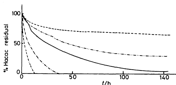
Figure 2. Plot of % residual Hacac versus time for different Cu(acac)_2 concentrations: [Hacac] 0.35M; [C_2N_2] 0.40M; [Cu(acac)_2] , ——— 4 \times 10^{-4}M ; — · — 8 \times 10^{-4}M ; — 1.2 \times 10^{-3}M ; — · — · — 5.7 \times 10^{-3}M ; [Hacac] 0.28M; [C_2N_2] 0.30M; [Cu(acac)_2] , — · — · — 5.7 \times 10^{-3}M ; — · — · — '0.1' M (analytical concentration)
