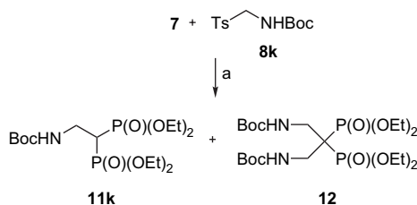
Scheme 3. Reagents and conditions: (a) NaH (2 equiv), -20^\circ\text{C} to -10^\circ\text{C} , 3 h, THF then satd aq \text{NH}_4\text{Cl} , -10^\circ\text{C} .
