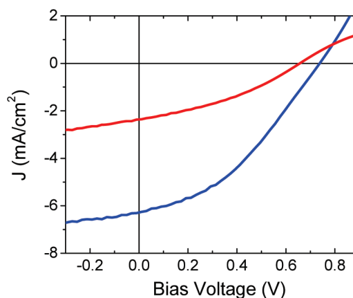
Figure 3. Performance of 9/10 :PC 60 BM cells. J – V characteristics under 100 mW/cm 2 white light illumination ( 9 in blue and 10 in red) annealed at 100 °C for 20 min.
