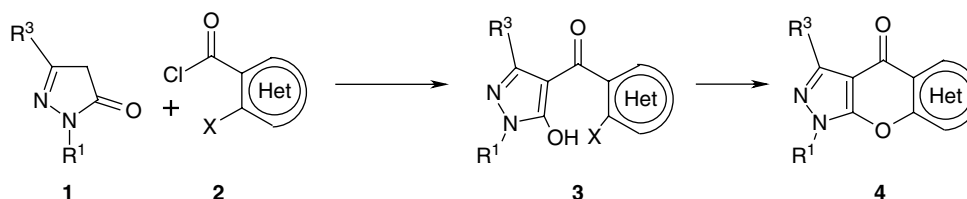
Scheme 1. Synthesis of [5,6]pyrano[2,3-c]pyrazol-4(1 H )-ones 4 .
