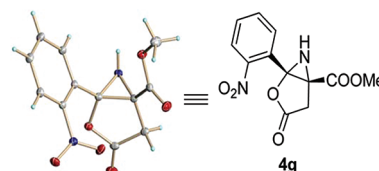
Figure 1. Crystal structure of the product 4g from the dirhodium(II)-catalyzed reaction between 1a and o -nitrobenzonitrile N -oxide 2g .
