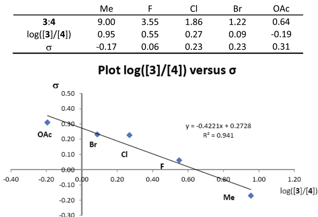
Figure 2. Plot of \log([3]/[4]) vs \sigma : \rho = -0.42 ( R^2 = 0.94 ).
