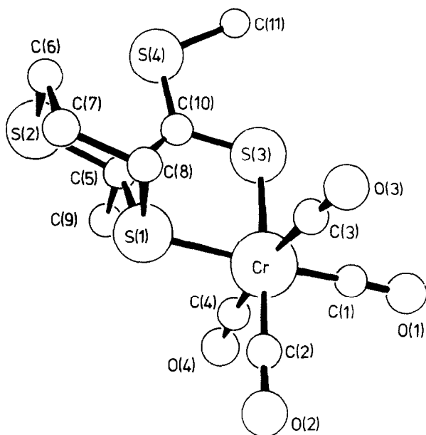
Fig. 2. A perspective view of \text{Cr}\{\text{SC}(\text{SMe})\text{C}(\text{CH}_3)\text{S}(\text{CH}_2)_3\text{S}\}(\text{CO})_4 ( A ) showing the atomic numbering.
