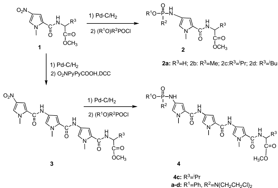
Synthetic route of nitrogen mustard/tripolypyrrole conjugate.
