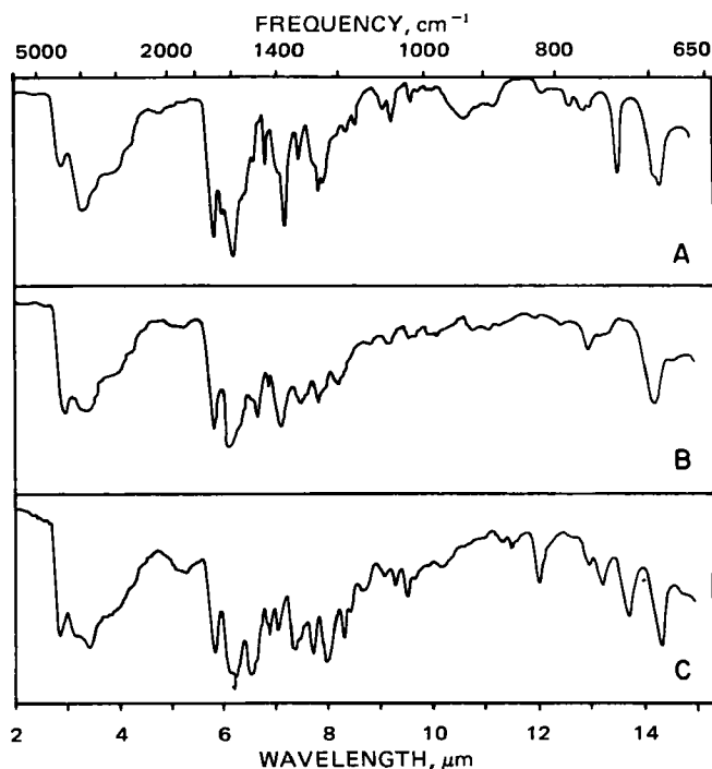
Figure 2 —IR spectra in KBr of DL-2-phenylglutamic acid (A), DL-3-phenyl-DL-glutamic acid (B), and DL-4-phenyl-DL-glutamic acid (C).
