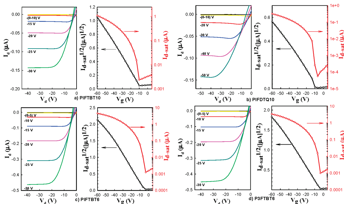
Figure 4. I_d - V_d curves of FET devices as a function of V_g (left), I_{d-sat} and I_{d-sat}^{1/2} vs V_g (right) based on spin-cast films for the polymers (a) PIFTBT10 , (b) PIFDTQ10 , (c) PIFTBT6 , and (d) P3FTBT6 .
