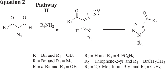
Scheme 1. Methods for preparing triazoles from \alpha -diazotrimines.
