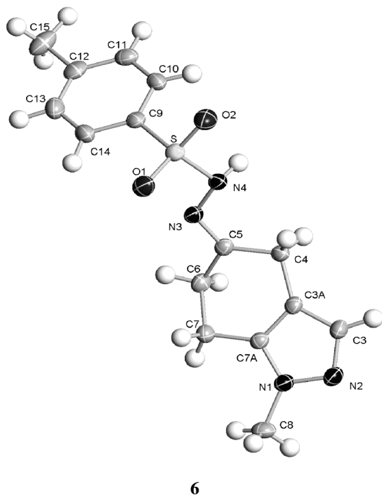
Figure 3. Ortep drawing of compound 6.
