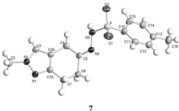
Figure 4. Ortep drawing of compound 7.
