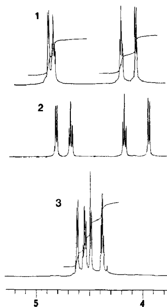
Fig. 1. ^1\text{H} NMR signals for aromatic protons in N -methyl-1,2,3,4-tetrahydroquinolinetricarbonylchromium (1), N -methylinolinetricarbonylchromium (2), N,N -dimethyltoluenetricarbonylchromium (3).
