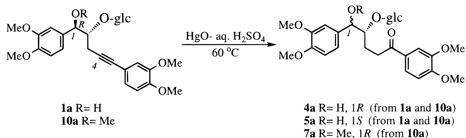
Figure 4. Hydration of tetra- O -methylnyasicoside and its 1- O -methyl derivative catalyzed by mercuric ion.
