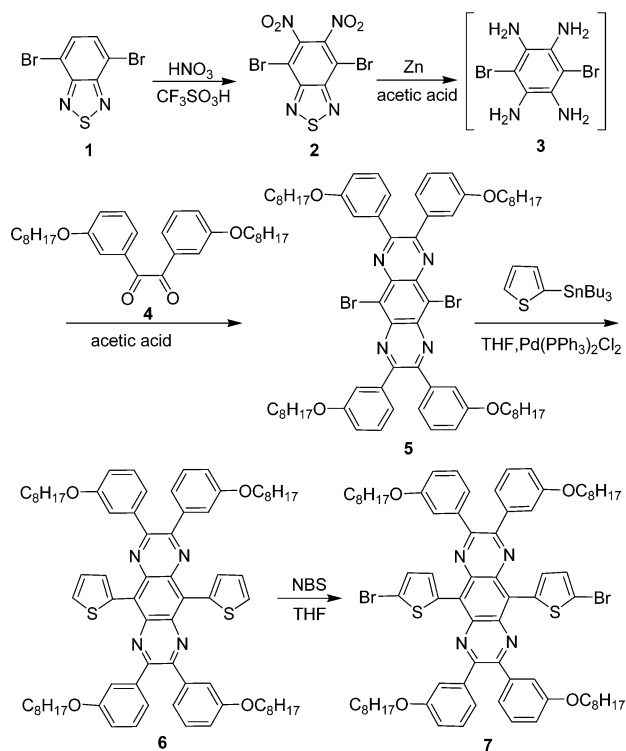
Scheme 1. Synthesis of the Two Monomers
