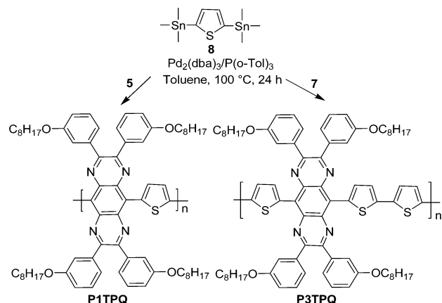
Scheme 2. Synthesis of the Two Polymers P1TPQ and P3TPQ
