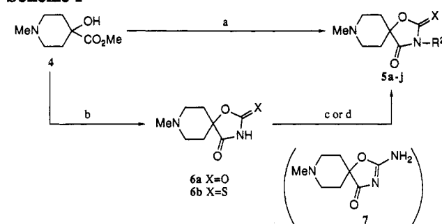
Scheme I a
