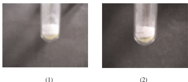
Fig.2 Change in state of two-layer of acridine and 3-methyl-1-phenyl-5-pyrazolone: (Upper part: 3-methyl-1-phenyl-5-pyrazolone, Lower part: acridine.) (1) initially; (2) after heating for 5hr at 50°.
