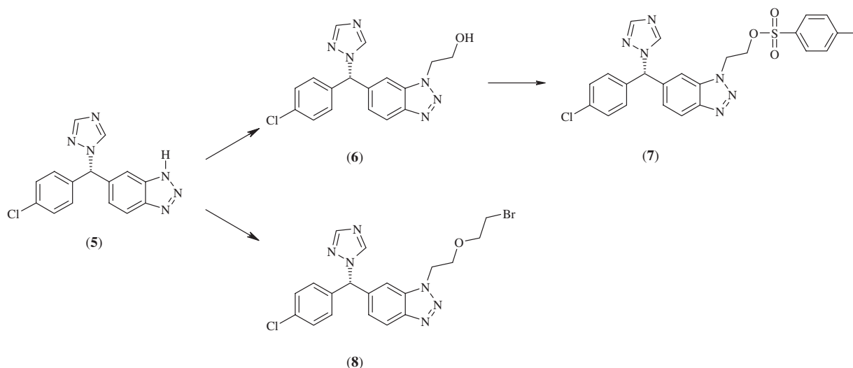
Scheme 3. Precursor synthesis.
