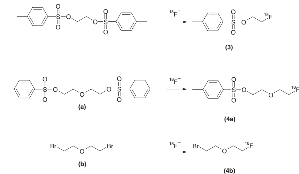
Scheme 1. ^{18}\text{F} -Labelled intermediates.
