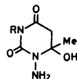
(7a) R = H (8a) R = Me
