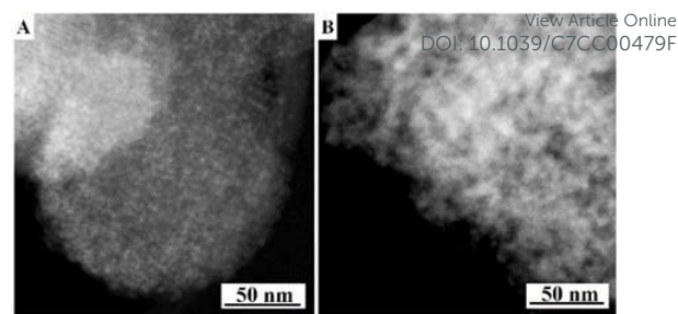
Fig. 3 STEM images of 20 wt% Cu supported AF-MCM-48 (A) and AF- \gamma -Al 2 O 3 (B).
