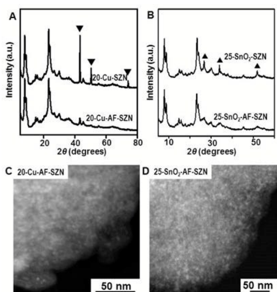
Fig. 2 (A,B) XRD patterns (bottom) and (C, D) STEM images of 20 wt% Cu and 25 wt% SnO 2 supported AF-SZN samples. (A,B) XRD patterns (top) of 20 wt% Cu and 25 wt% SnO 2 supported SZN samples are also displayed for comparison. The XRD peaks of metallic Cu and SnO 2 are marked with an inverted triangle and a triangle.
