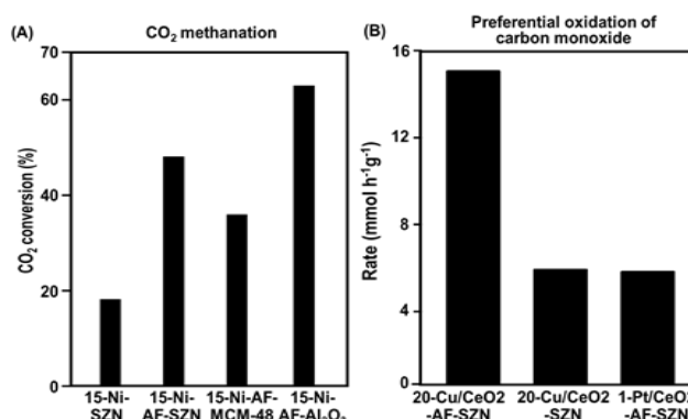
Fig. 4 (A) Conversion of CO 2 to methane over Ni supported on various kinds of support materials (Reaction conditions: GHSV = 17000 h -1 , H 2 :CO 2 molar ratio = 4:1, 300 °C, 1 atm). (B) Rate of CO conversion over Cu/CeO 2 supported catalyst and Pt/CeO 2 supported catalyst (reaction conditions: 130 °C, 50 mg of catalyst, 73 mL min -1 of gas flow rate with a molar composition of CO/O 2 /H 2 /He = 0.7/0.8/63.0/34.9, 1 atm).
