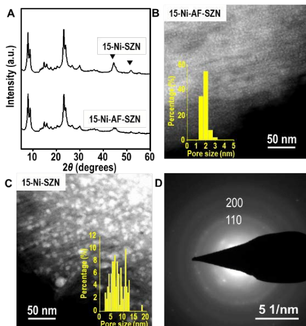
Fig. 1 XRD pattern (A, bottom), STEM image (B), and SAED pattern (D) for the 15 wt% Ni-supported AF-SZN sample. The XRD pattern (A, top) and STEM image (C) for the 15 wt% Ni-supported SZN sample are displayed for comparison. The XRD peaks of metallic Ni are marked with an inverted triangle.
