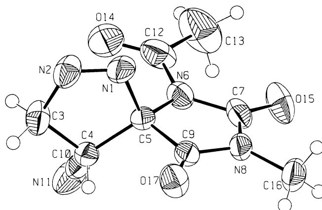
Fig. 4. ORTEP View of the asymmetric unit of compound 12 with labelling (arbitrary) of non-H-atoms. Ellipsoids are at 50% probability level.
