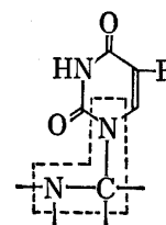
Fig. 1. Geminal Diamine Moiety of 5-Fluorouracil Derivatives
