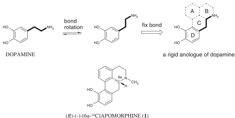
Scheme 1. Chemical structures of (R)-(-)-[6a- 14 C]apomorphine (1) and dopamine
