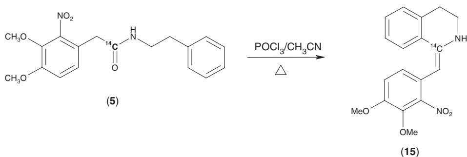
Scheme 6. The Bischler–Napieralski exocyclic product (15)
