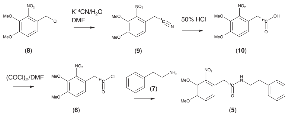
Scheme 3. Synthetic route to 3,4-dimethoxy-2-nitrophenyl- N -phenethyl [carboxyl- 14 C]acetamide (5)
