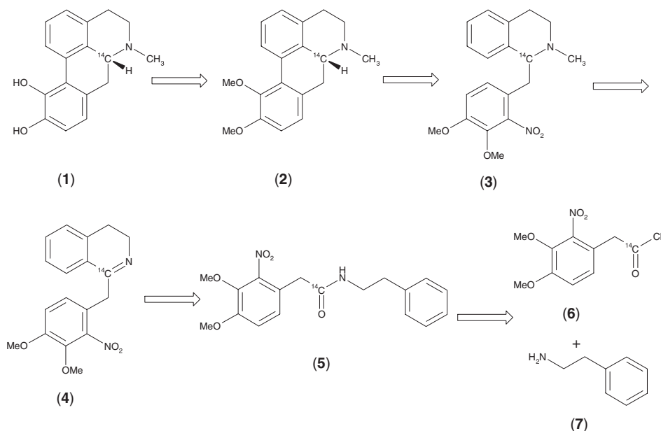
Scheme 2. Retrosynthetic analysis of (R)-(-)-[6a- 14 C]apomorphine (1)
