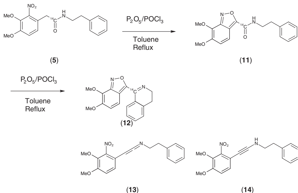
Scheme 5. Bischler–Napieralski dehydration products
