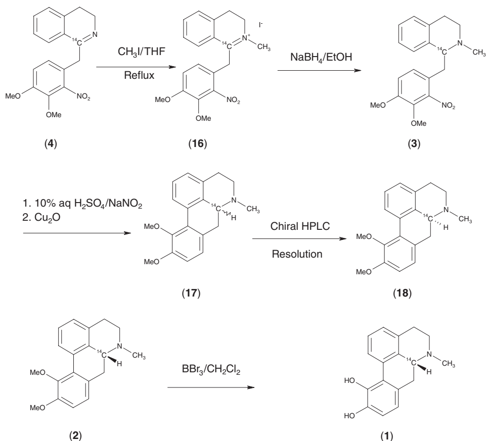
Scheme 7. Radiosynthesis of ( R )-(-)-[6a- ^{14}\text{C} ]apomorphine (1)
