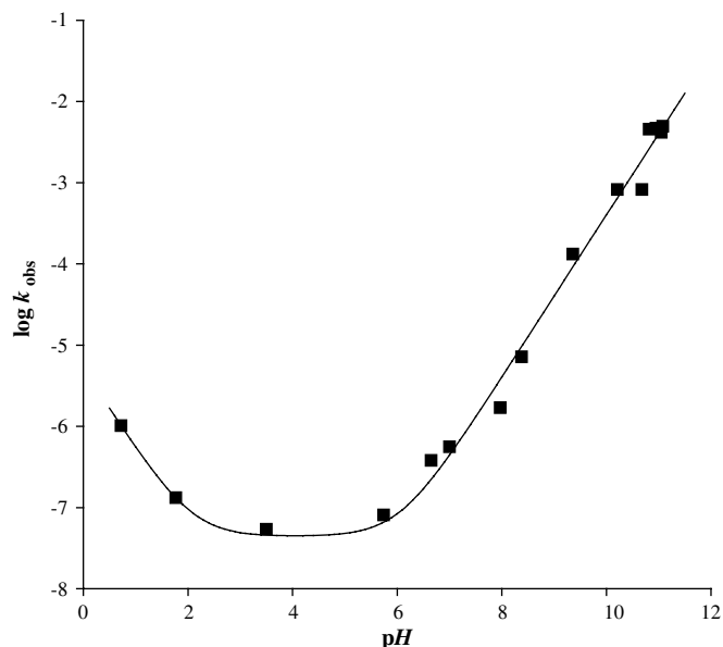
Fig. 3. pH-rate profile for compound 6a . The points are experimental, the curve is the best fit using k_{\text{OH}} 5.7 \text{ M}^{-1} \text{ s}^{-1} , k_{\text{H}_2\text{O}} 4.4 \times 10^{-8} \text{ s}^{-1} and k_{\text{H}^+} 5.17 \times 10^{-5} \text{ M}^{-1} \text{ s}^{-1} .
