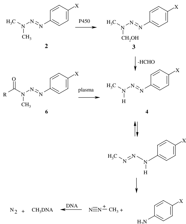
Fig. 1. Metabolism pathways for 1-aryl-3,3-dimethyltriazenes and 3-aminoacyl-1-aryl-3-methyltriazenes.
