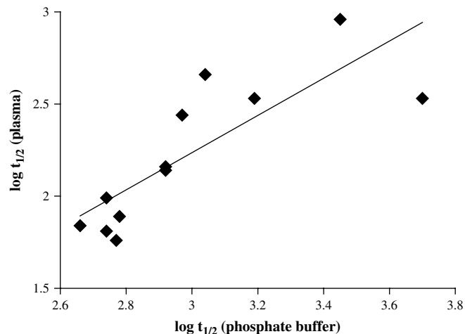
Fig. 5. Correlation of the plasma half-lives with the phosphate buffer half-lives for compounds 6a–l .
