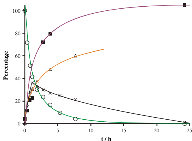
Fig. 2. Time course for the hydrolysis of 6g in 80% human plasma at 37 °C: ○, 6g ; ■, N -benzoyl-( S )-alanine; ×, 4 ; △, corresponding aniline.
