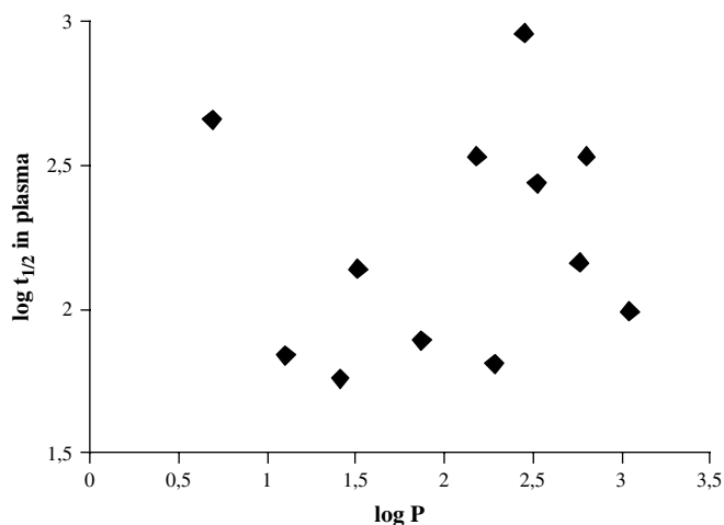
Fig. 6. Plot of the plasma half-lives versus lipophilicity for compounds 6a–l .
