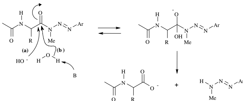
Fig. 7. Pathways of the hydroxide (a) and general base (b) catalysed hydrolyses of triazene prodrugs 6a–l .
