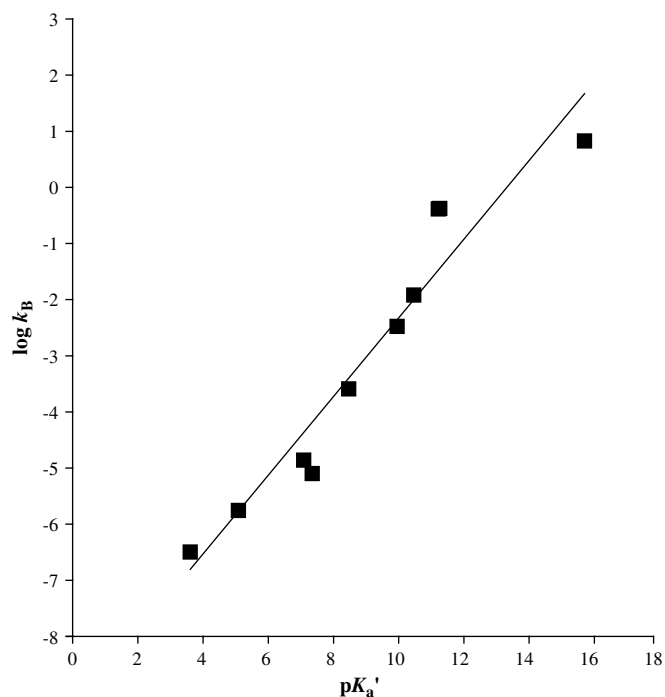
Fig. 4. Brønsted plot for compound 6a .
