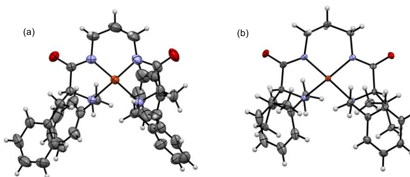
Figure 5. X-ray crystal structures of \text{Cu}^{2+} complexes 5a (a) and 6a (b). Ellipsoids represented at the 50% probability level.
