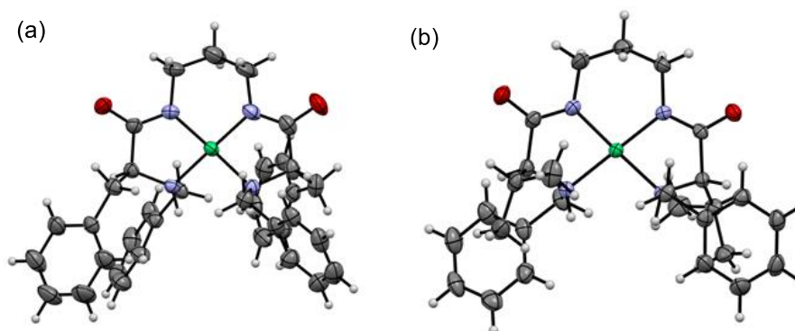
Figure 6. X-ray crystal structure of complexes 5b (a) and 6b (b). Ellipsoids represented at the 50% probability level.
