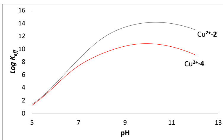
Figure 4. Plot of the effective conditional constants v. pH for the systems \text{Cu}^{2+}\cdot\mathbf{2} and \text{Cu}^{2+}\cdot\mathbf{4} in 0.1 M NaCl in \text{H}_2\text{O}/\text{CH}_3\text{CN} 7/3 v/v, at 298.1 \pm 0.1 K.
