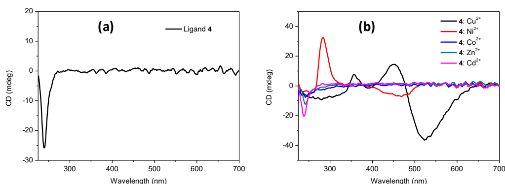
Figure 2. (a) CD spectra for ligand 4 in basic media (2 equiv. of NaOH). (b) CD spectra for ligand 4 in basic media (2 equiv. of NaOH) in the presence of 1 equivalent of different M 2+ metals. In all cases the solvent was MeOH/H 2 O 80/20 (v/v) and the concentration of the metal and the ligand 2.5 mM.
