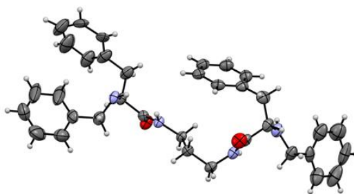
Figure 1. X-ray crystal structure of ligand 3 .
