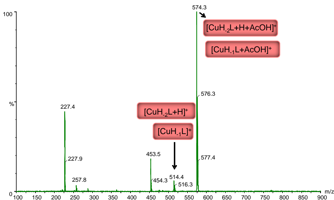
Figure 3. ESI + -MS of compound 4 (5 mM) in the presence of 1 equiv. of Cu(OAc) 2 in MeOH/H 2 O 80/20, v/v.
