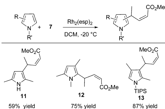
Figure 2. Vinylogous reaction of 7 with pyrroles.
