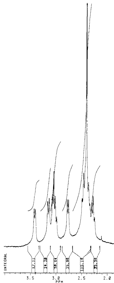
Figure 1. The piperazino proton signals in the 400-MHz nuclear magnetic resonance spectrum of 5-methylene-10-(4-methylpiperazino)-5H-dibenzo[a,d]cycloheptene ( 5a ) in chloroform- d at -50^{\circ}\text{C} .
