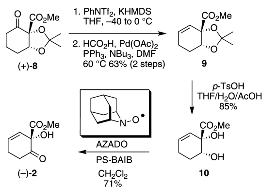
Scheme 2. Synthesis of Monomer 2
